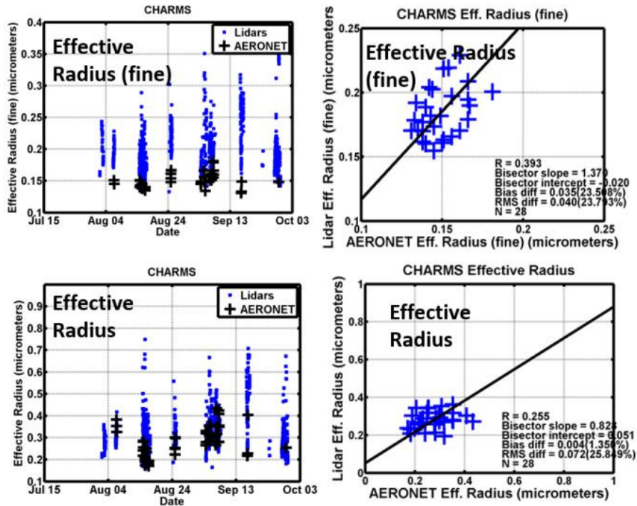
Figure 13. Same as Figure 12 except for comparison of fine (top) and total (bottom) effective radii from AA+TiARA and AERONET retrievals.
