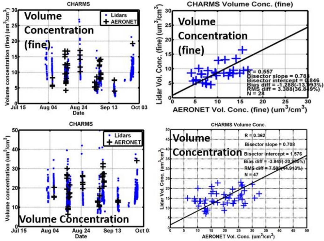
Figure 11. Same as Figure 10 except for comparison of fine (top) and total (bottom) volume concentrations from AA+TiARA and AERONET retrievals.
