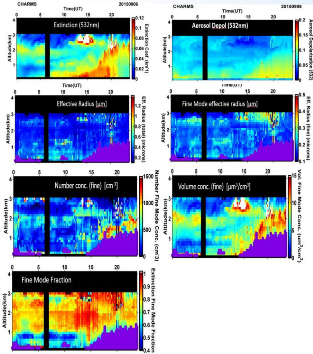
Figure 5. Same as Figure 4 except for AA+TiARA retrieval results. Temporal resolution is 10 minutes and vertical resolution is 120 m. Regions shaded in purple are when aerosol depolarization (532 nm) exceeds 0.1 such that non-spherical aerosols contribute significantly to aerosol backscatter and extinction.
