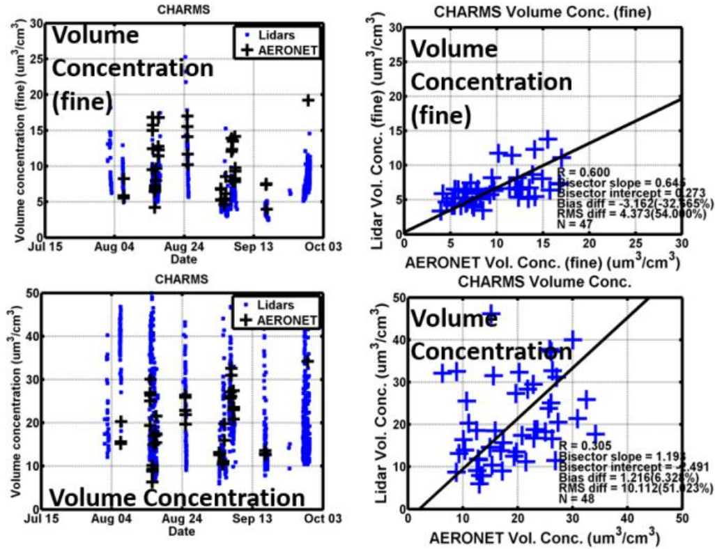
Figure 10. Comparison of fine (top) and total (bottom) volume concentrations from TiARA and AERONET retrievals.
