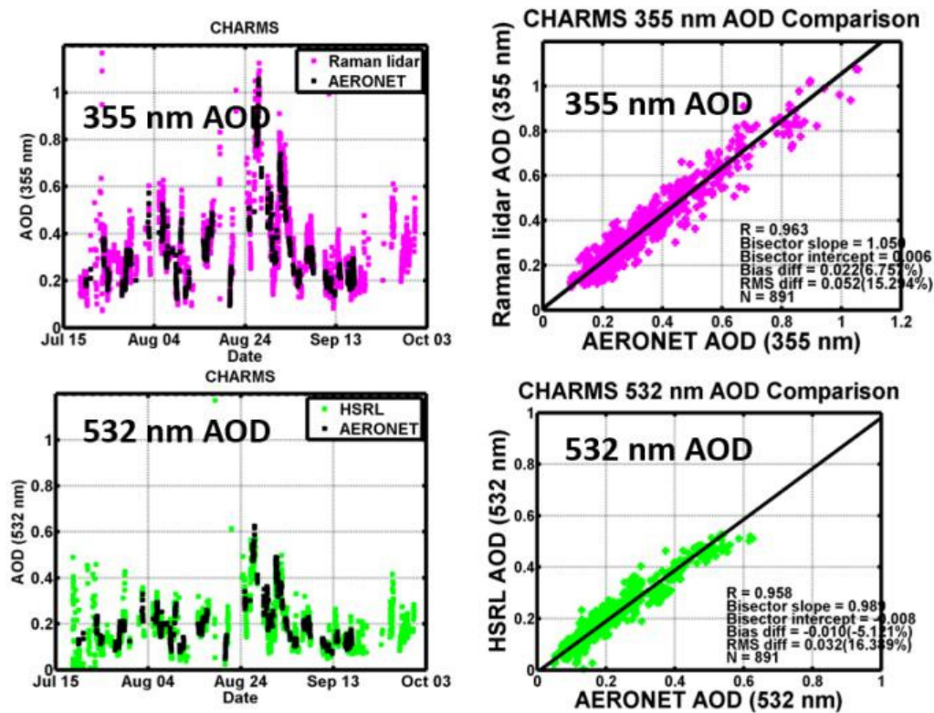
Figure 7. Comparison of aerosol optical depth (AOD) derived from the CHARMS measurements and AERONET data.
