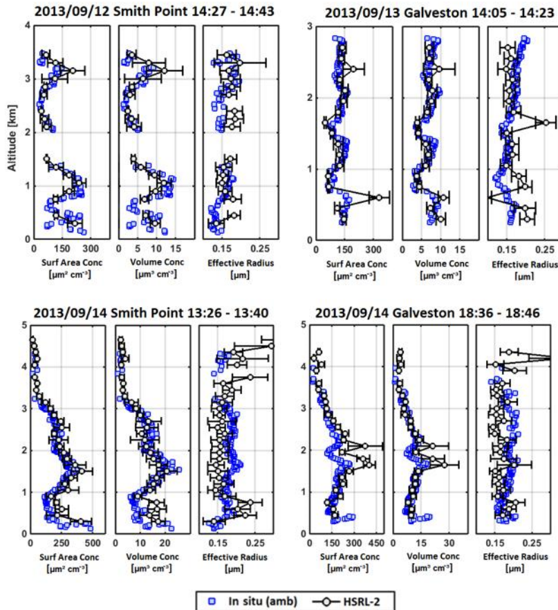
Figure 6. Comparison of TiARA aerosol retrieval results derived using NASA LaRC airborne HSRL measurements and airborne in situ data collected over the Houston, Texas region during the NASA DISCOVER-AQ mission. HSRL-2 retrievals are shown in black and in situ results are shown in blue (from Sawamura et al. 2017).
