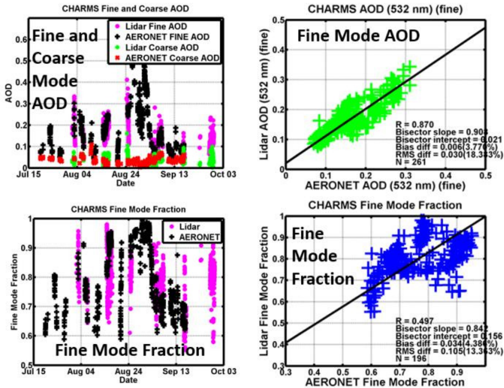
Figure 9. Same as Figure 8 except comparison of fine- and coarse-mode AOD and fine-mode fraction from AA+TiARA and AERONET SDA retrievals.
