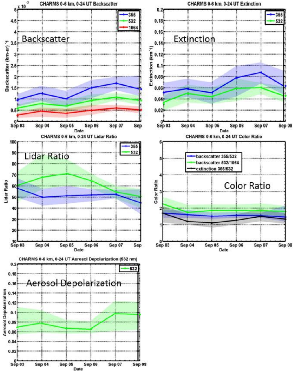
Figure 2. Same as for Figure 1 except for a subset of days (September 3-8) that use 1064 nm aerosol backscatter profiles computed using the revised calibration method.
