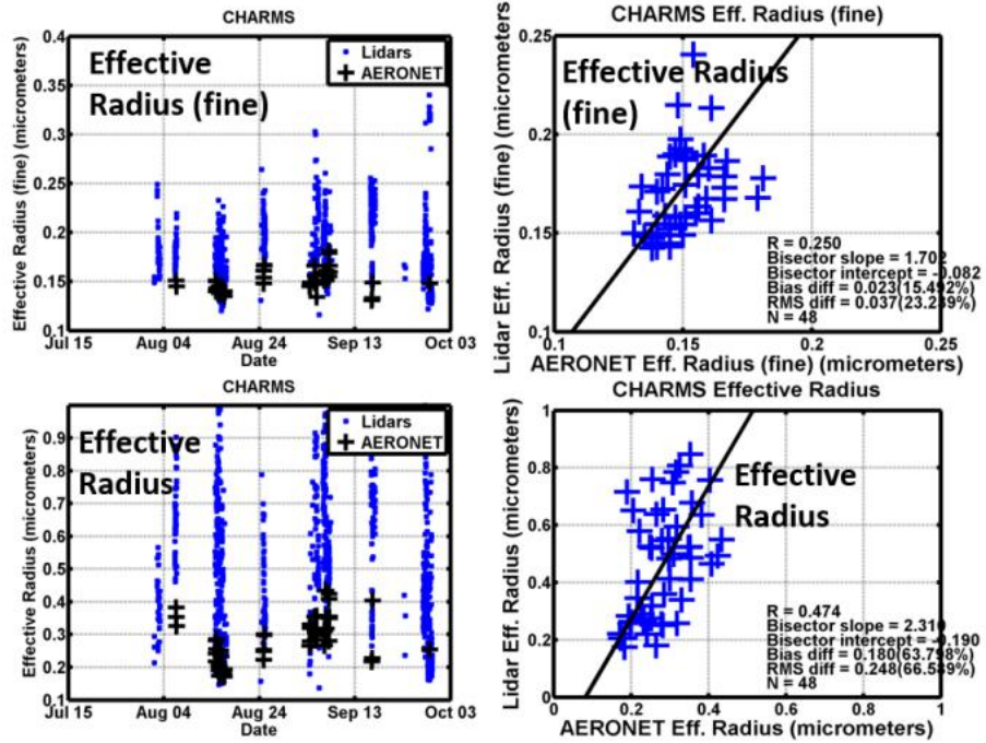
Figure 12. Comparison of fine (top) and total (bottom) effective radii from TiARA and AERONET retrievals.
