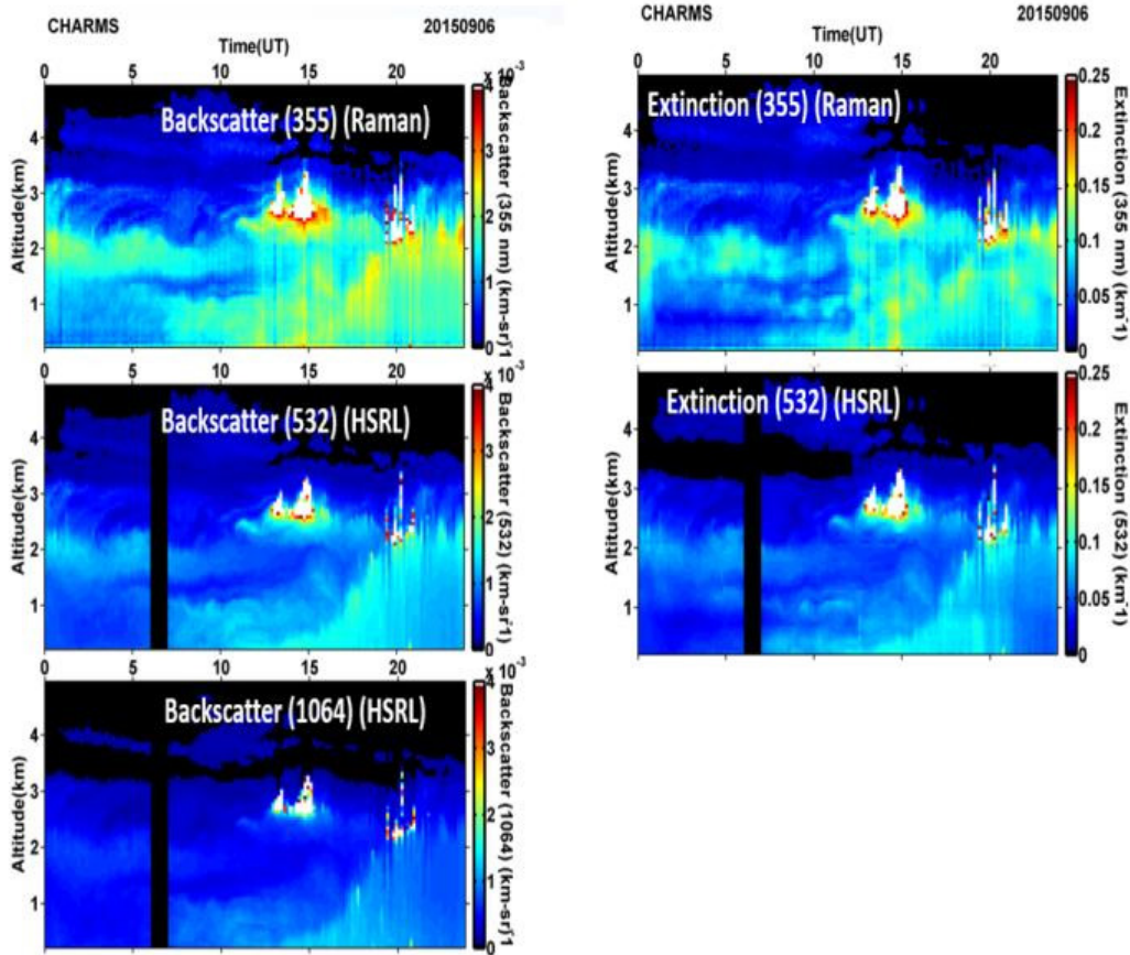
Figure 3. Example “ 3\beta+2\alpha ” data set for September 6, 2015. Temporal resolution is 10 minutes and vertical resolution is 60 m.
