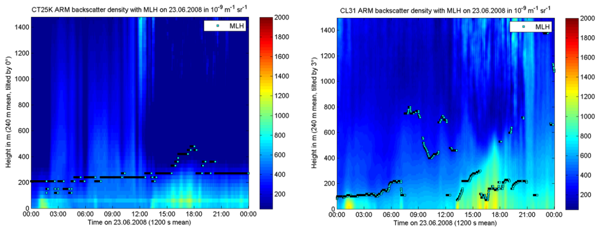
Figure 2. Backscatter density in 10^{-9} \text{ m}^{-1} \text{ sr}^{-1} with mixing-layer-height in m from Vaisala CT25K and CL31 Ceilometers on 06/23/08 at SGP.
