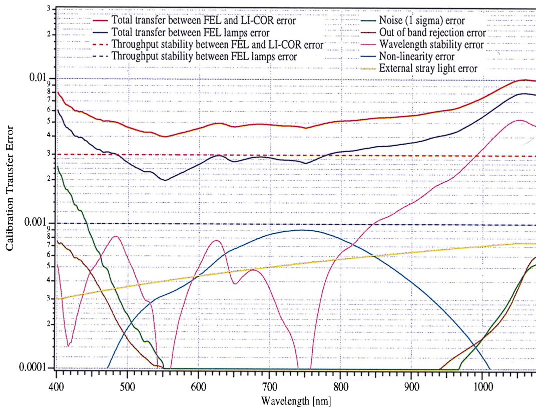
Fig. 7. Sources of fractional error that arise in transferring calibrations within the laboratory between spectral irradiance standards.
