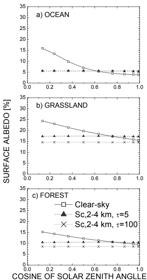
Figure 2. Dependence of surface albedo on atmospheric conditions.
