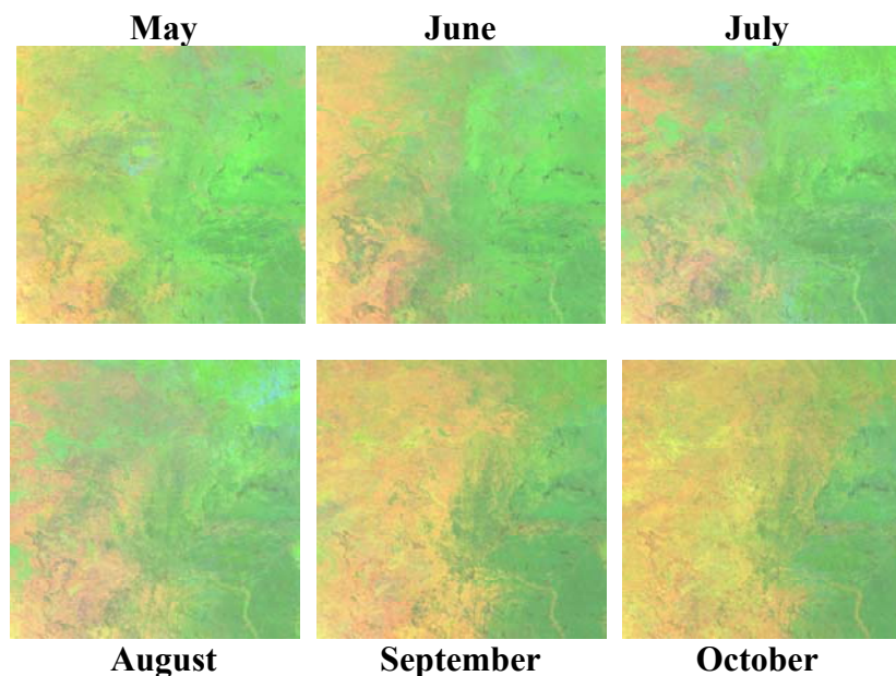
Figure 3. Surface reflectance over SGP area derived from normalized AVHRR observations in channels 1, 2, and 3 for May through October 2000.
