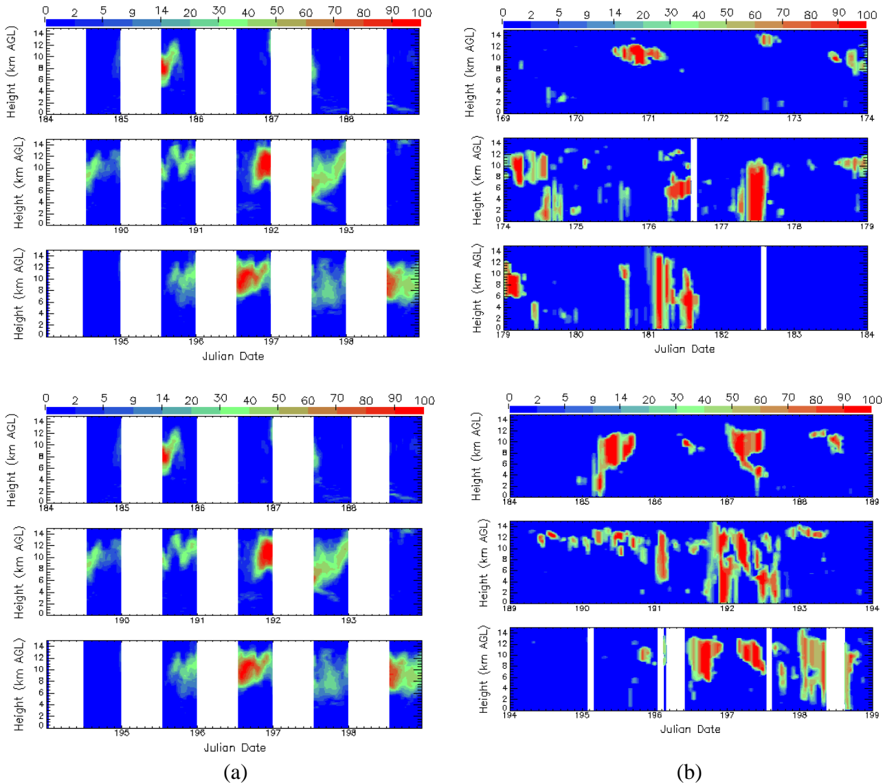
Figure 3. Cloud fractions during Case 3 from (a) averages of Cloud and Radiation Testbed (CART)-wide estimates of cloud heights and cloud thicknesses from Minnis analyses of GOES-8 radiance data, and (b) cloud occurrence frequency analyses of MMCR data at the SGP central facility.
