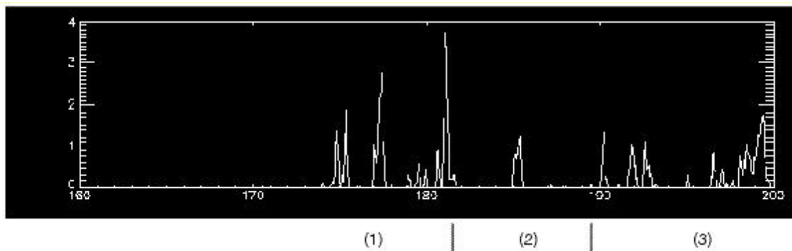
Figure 1. Hourly precipitation rates (mm/hr) over the SGP SCM domain during the Summer 1997 SCM IOP (Julian days 169-199), also known as Case 3, as derived from National Weather Service (NWS) Weather Surveillance Radar-88 Dopplers (WSR-88D) radar data.
