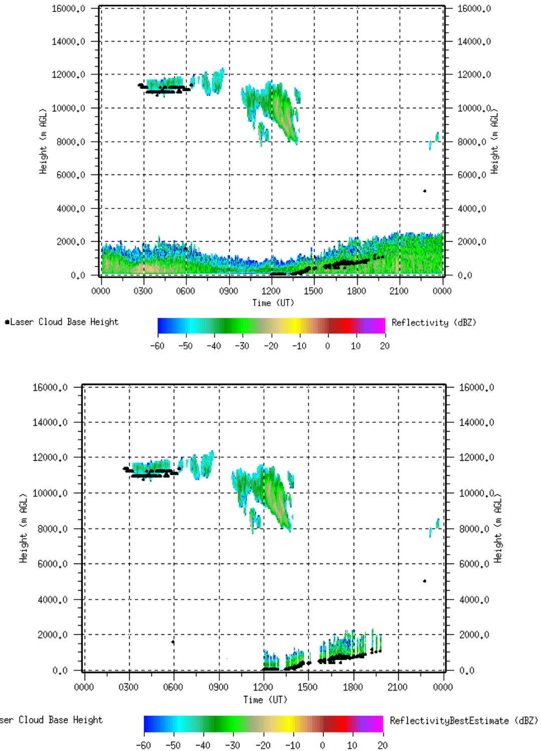
Figure 7. MOCR reflectivities (a) before and (b) after the application of algorithms for the removal of insects and other signal-contaminating objects in the boundary layer.
