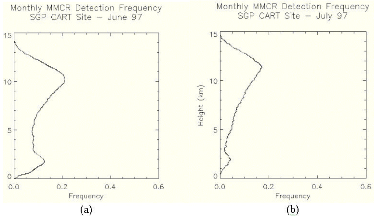
Figure 4. Monthly cloud-detection frequencies at the SGP central facility from MMCR data for (a) June 1997 and (b) July 1997.
