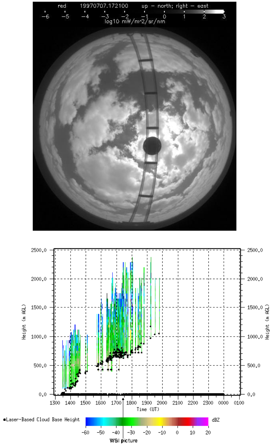
Figure 8. (a) Whole sky image of boundary layer clouds, and (b) cloud heights, as established by MMCR and ceilometer data (arrow points to the time at which the WSI image was taken).
