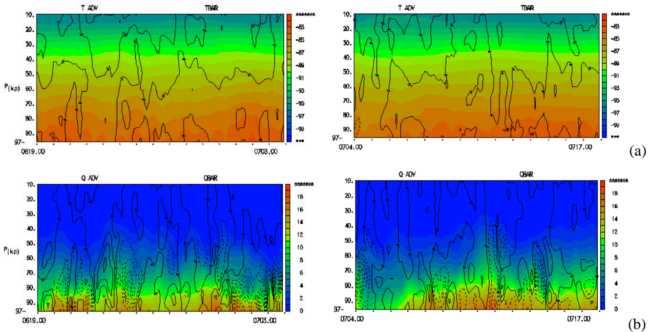
Figure 2. Time-height observations and analyses of (a) mean temperatures in degrees Celsius (colors) and their advective tendencies (lines), and (b) mean water vapor mixing ratios in g/kg (colors) and their advective tendencies (lines) for Case 3, based on Zhang’s variational analysis techniques.
