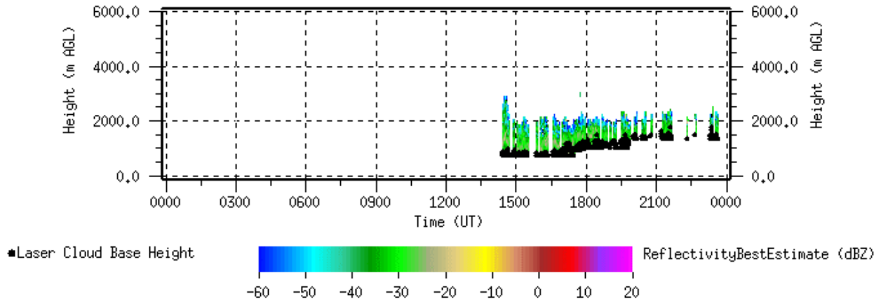
Figure 6. MMCR reflectivities (colors) and ceilometer cloud-base heights (black circles) for SGP boundary layer clouds on June 21, 1997.
